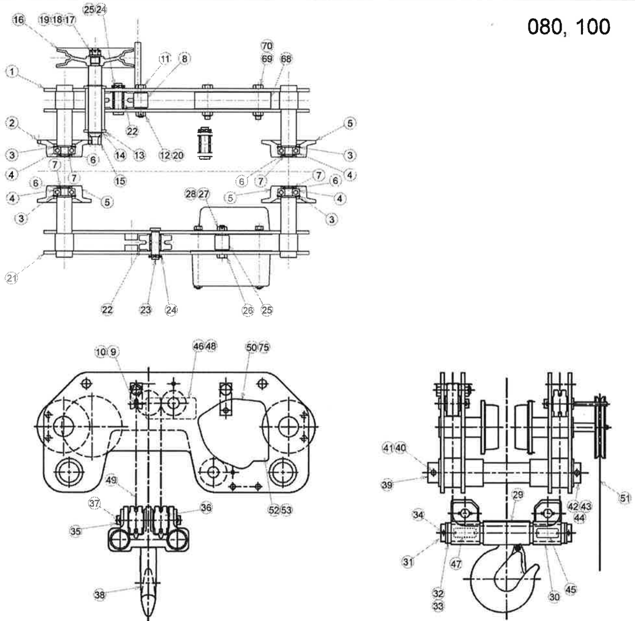
Figure 9-2-1 SHB (8 to 10 Ton)
