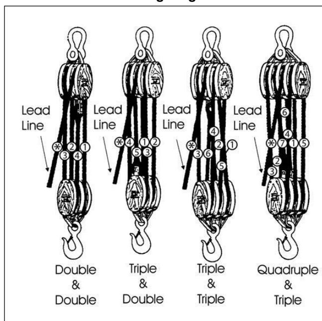
Reeving Diagram
